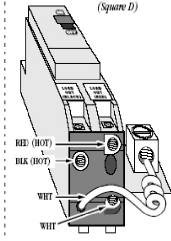
Bottom View of G.F.C.I. (Square D)
