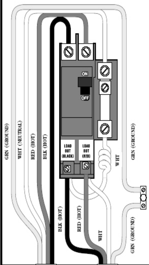
Front View of G.F.C.I. (Square D)
